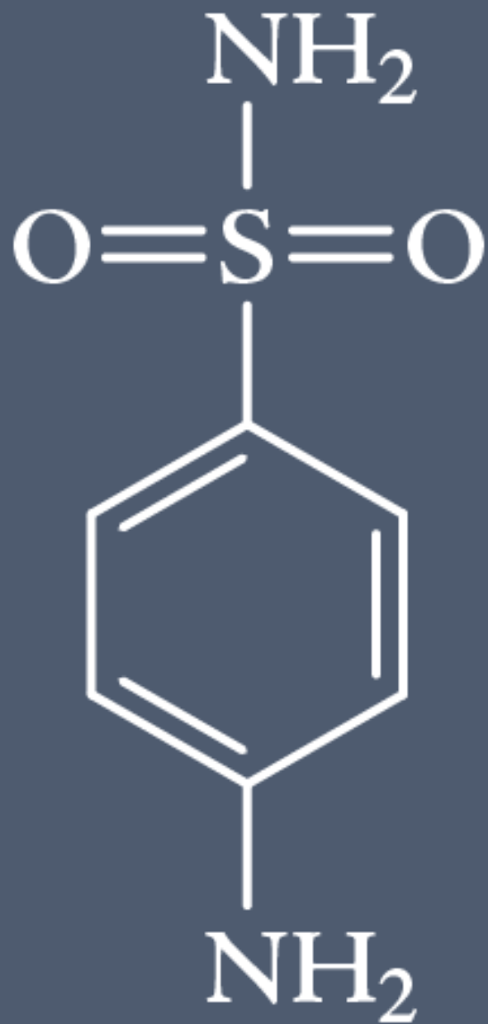
Sulfanilamide
